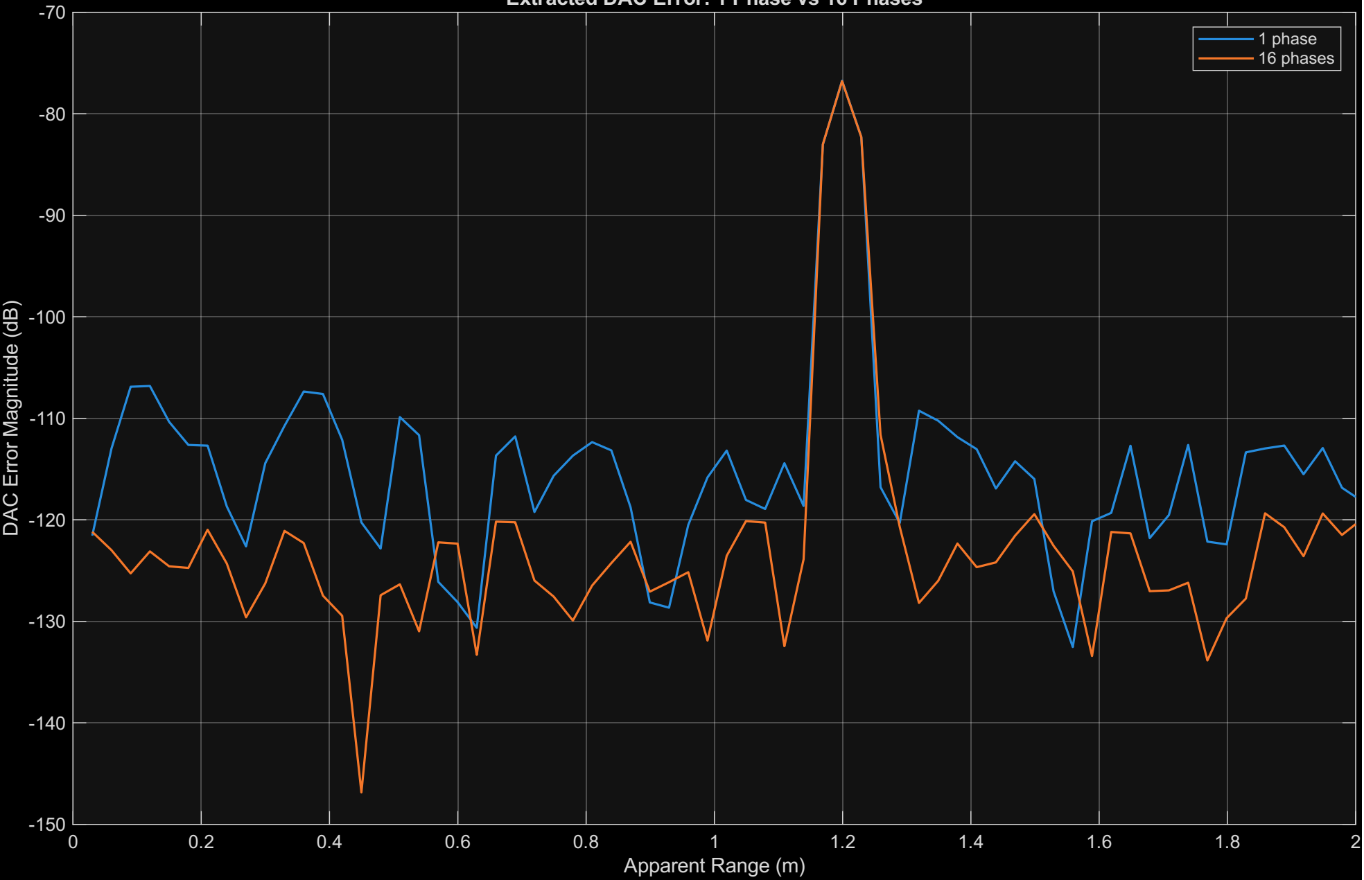
Extracted DAC Error: 1 Phase vs 16 Phases
